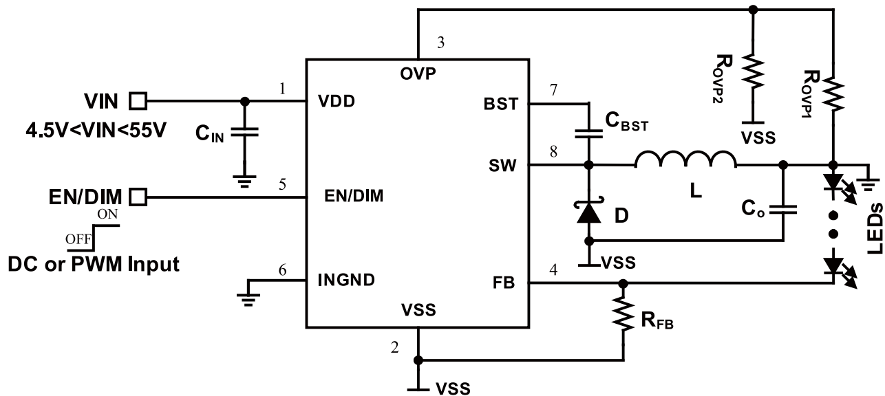
Figure 4: White LED Driver Step-Up/Down Application
